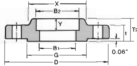
SOCKET WELDING
