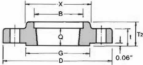
THREADED
