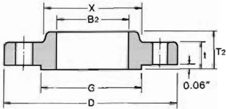
SLIP-ON
