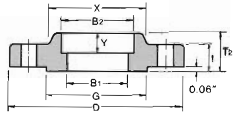
SOCKET WELDING
