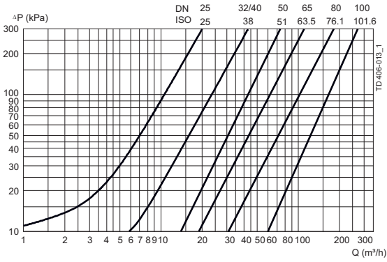
Fig.1. Note! For the diagram the following applies: Medium: Water (68°F). Measurement: In accordance with VDI 2173.
